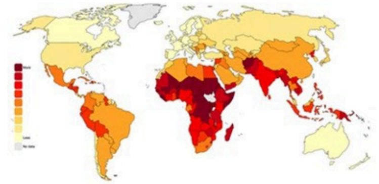
Multi-dimensional climate vulnerability (ND-GAIN)
