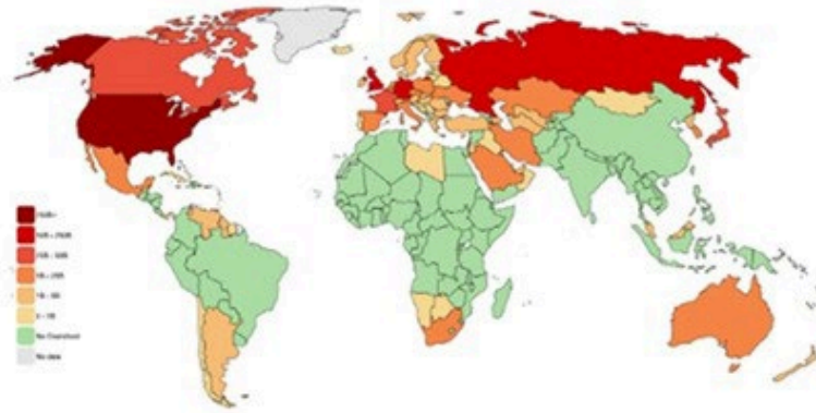
Overshoot emissions (Lancet Planetary Health)
